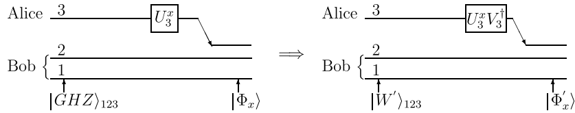
Figure 2. Superdense coding of two classical bits: when the shared resource is changed from |\text{GHZ}\rangle_{123} to |W'\rangle_{123} = (V_{12} \otimes V_3)|\text{GHZ}\rangle_{123} , then the operators applied by Alice are changed from \{U_3^x\} to \{U_3^x V_3^\dagger\} , and the states resulted at Bob' end are changed from \{|\Phi_x\rangle\} to \{|\Phi'_x\rangle : (V_{12} \otimes I_3)|\Phi_x\rangle\} .
