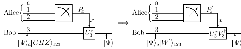
Figure 1. Teleportation of state |\Psi\rangle : when the shared resource is changed from |\text{GHZ}\rangle_{123} to |W'\rangle_{123} = (V_{12} \otimes V_3)|\text{GHZ}\rangle_{123} , then the measurement projectors made by Alice are changed from \{P_x\} to \{P'_x : (I_a \otimes V_{12})P_x(I_a \otimes V_{12}^\dagger)\} , and the operators applied by Bob are changed from \{U_3^x\} to \{U_3^x V_3^\dagger\} .
