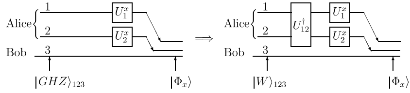
Figure 3. Change the channel from |GHZ\rangle_{123} to |W\rangle_{123} for superdense coding of three classical bits.
